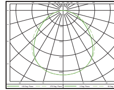
CLF22-S1-C-UV / Lumens: 5382
