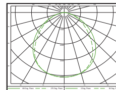
CLF14-H1-C-UV / Lumens: 10030
